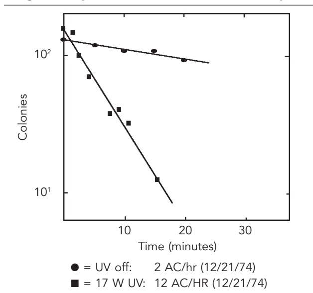
Figure 2. Disappearance of aerosolized bacillus Calmette-Guérin (BCG) from room air with and without upper room ultraviolet (UVGI) irradiation using one suspended fixture with one 17 W lamp.
